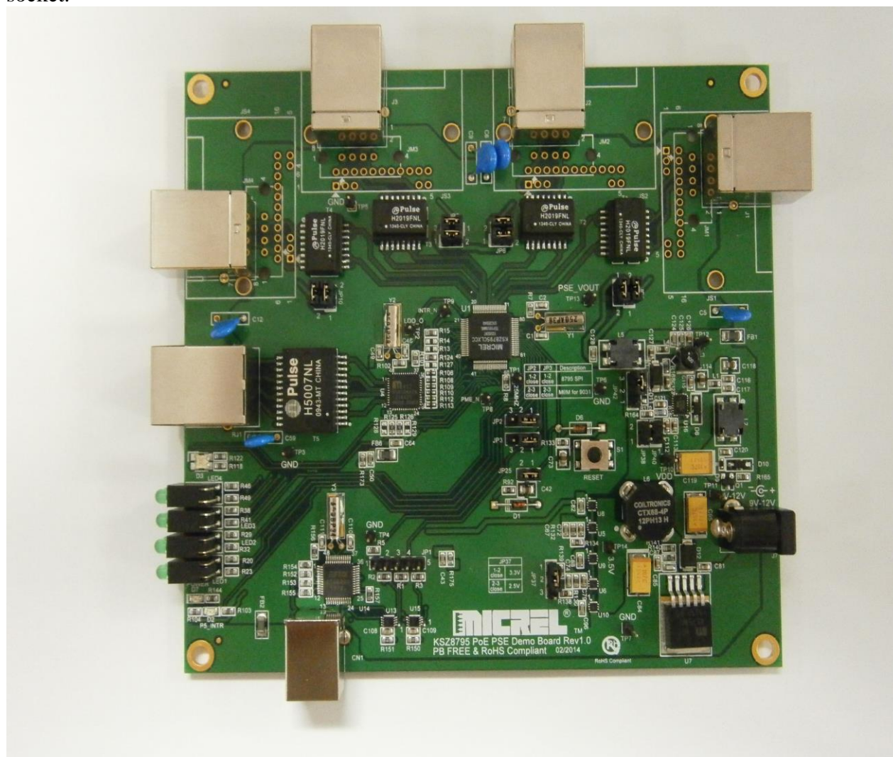
Figure 1 KSZ8795-POE-EVAL Board
